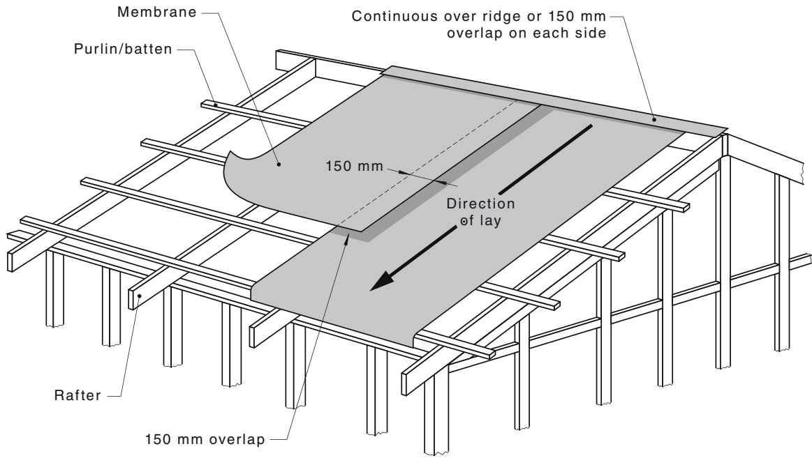
(a) Over battens—Option A
