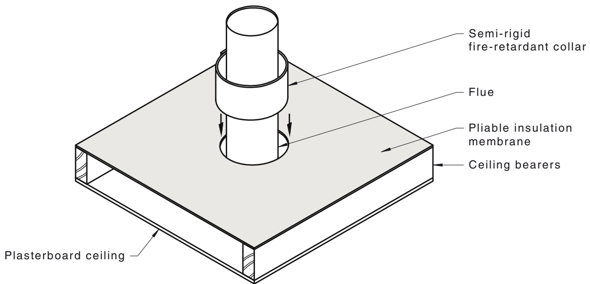
(a) Collar insert—Step 1
