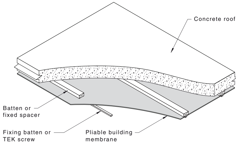
FIGURE 3.10(B) EXAMPLE OF PLIABLE BUILDING MEMBRANE UNDER A SUSPENDED CONCRETE SLAB
