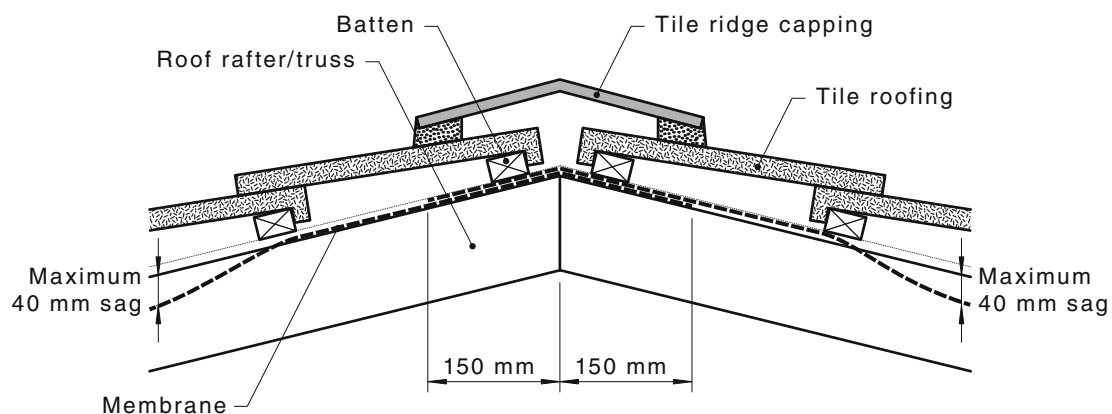
FIGURE 3.5.5 TREATMENT OF TILED ROOF AT RIDGES
