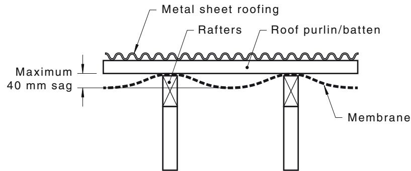
FIGURE 3.4.2 INSTALLATION OF MEMBRANE AS REFLECTIVE INSULATION— UNDER BATTENS
