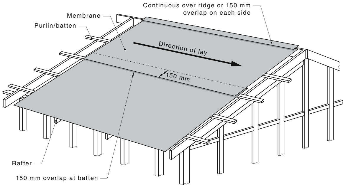
(b) Over battens—Option B
