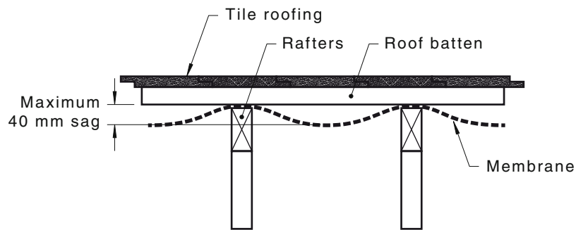
FIGURE 3.5.1(B) INSTALLATION OF MEMBRANE UNDER BATTENS WITH SAG
