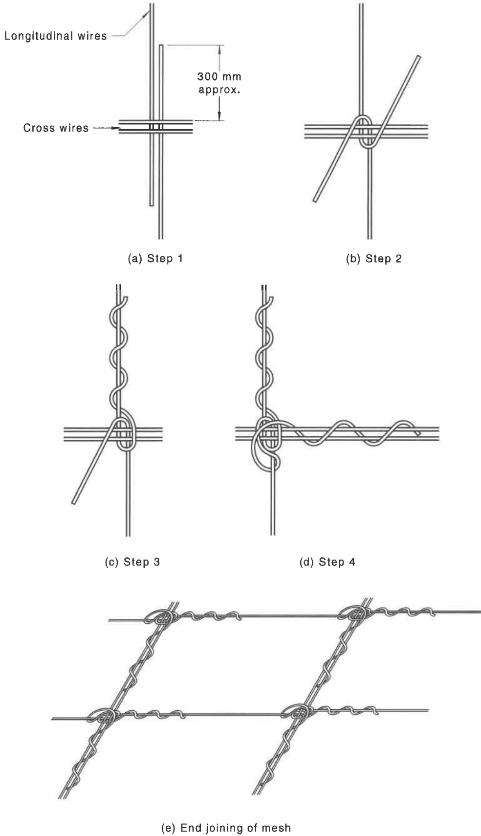
FIGURE 2 LONGITUDINAL WIRE JOINING
